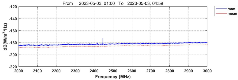
Fig.6 RFI scan of 2000-3000MHz in nighttime.
